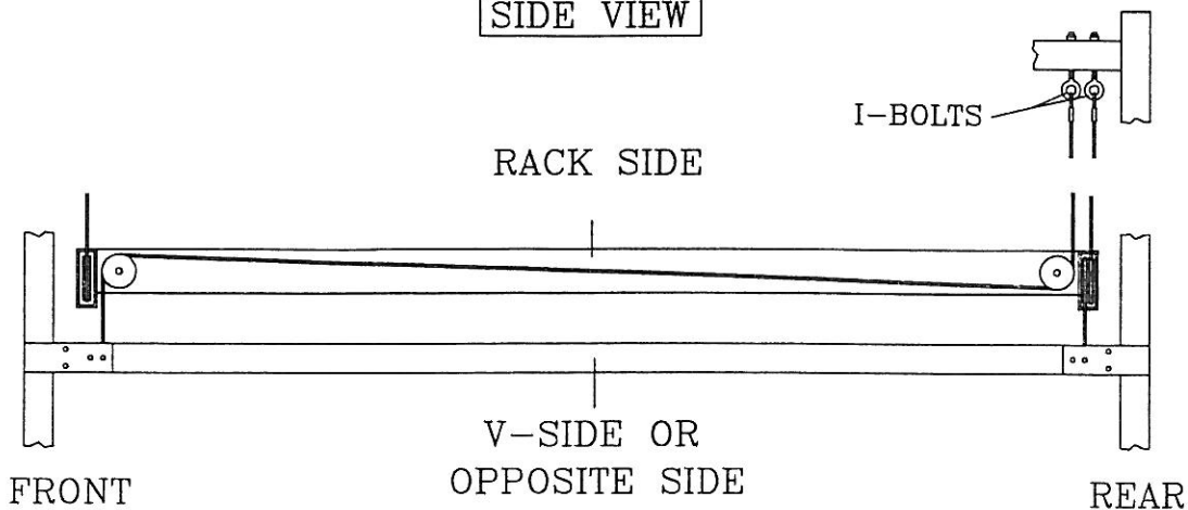
SIDE VIEW
